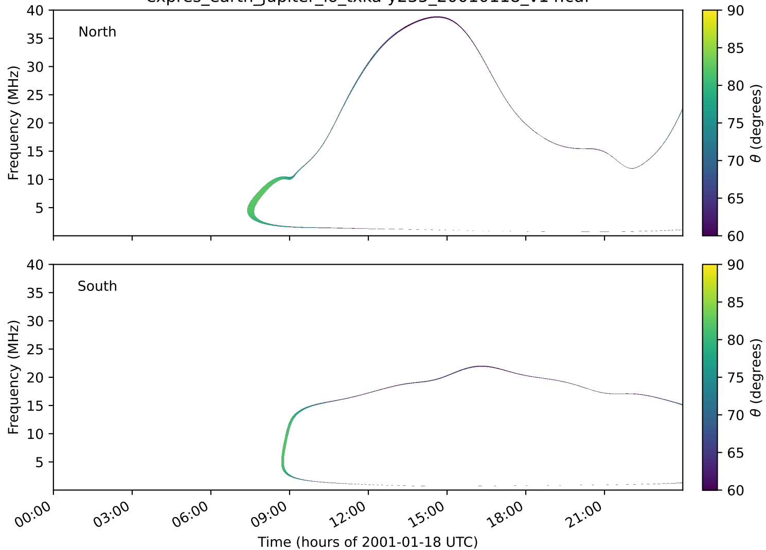
expres_earth_jupiter_io_txka-y235_20010118_v14.cdf
