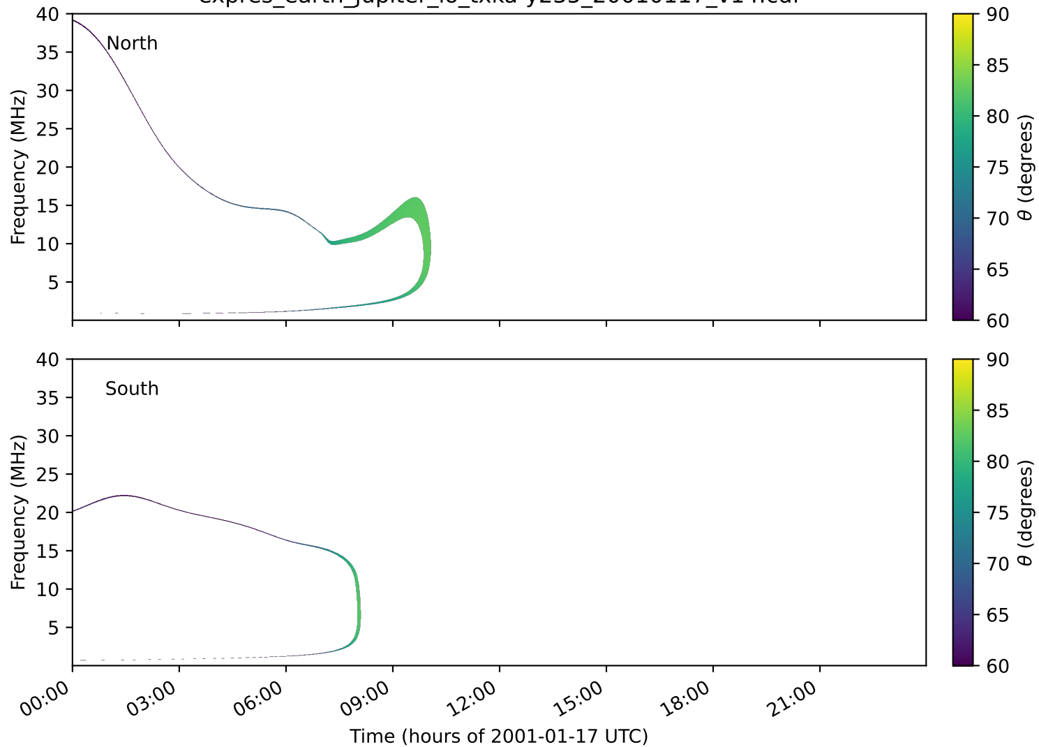
expres_earth_jupiter_io_txka-y235_20010117_v14.cdf
