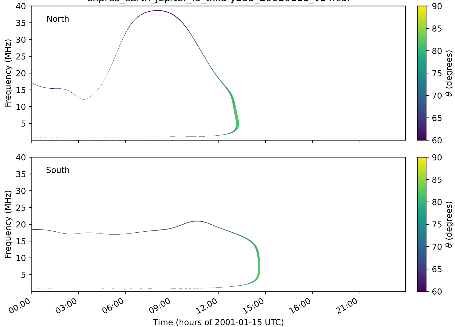
expres_earth_jupiter_io_txka-y235_20010115_v14.cdf
