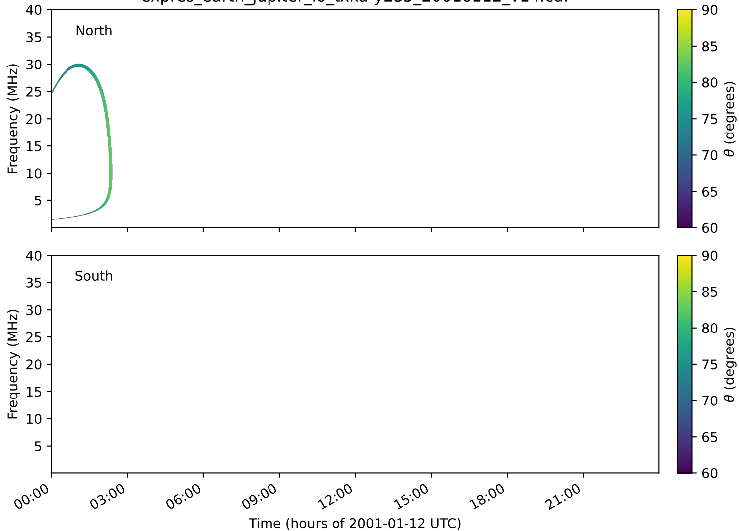
expres_earth_jupiter_io_txka-y235_20010112_v14.cdf
