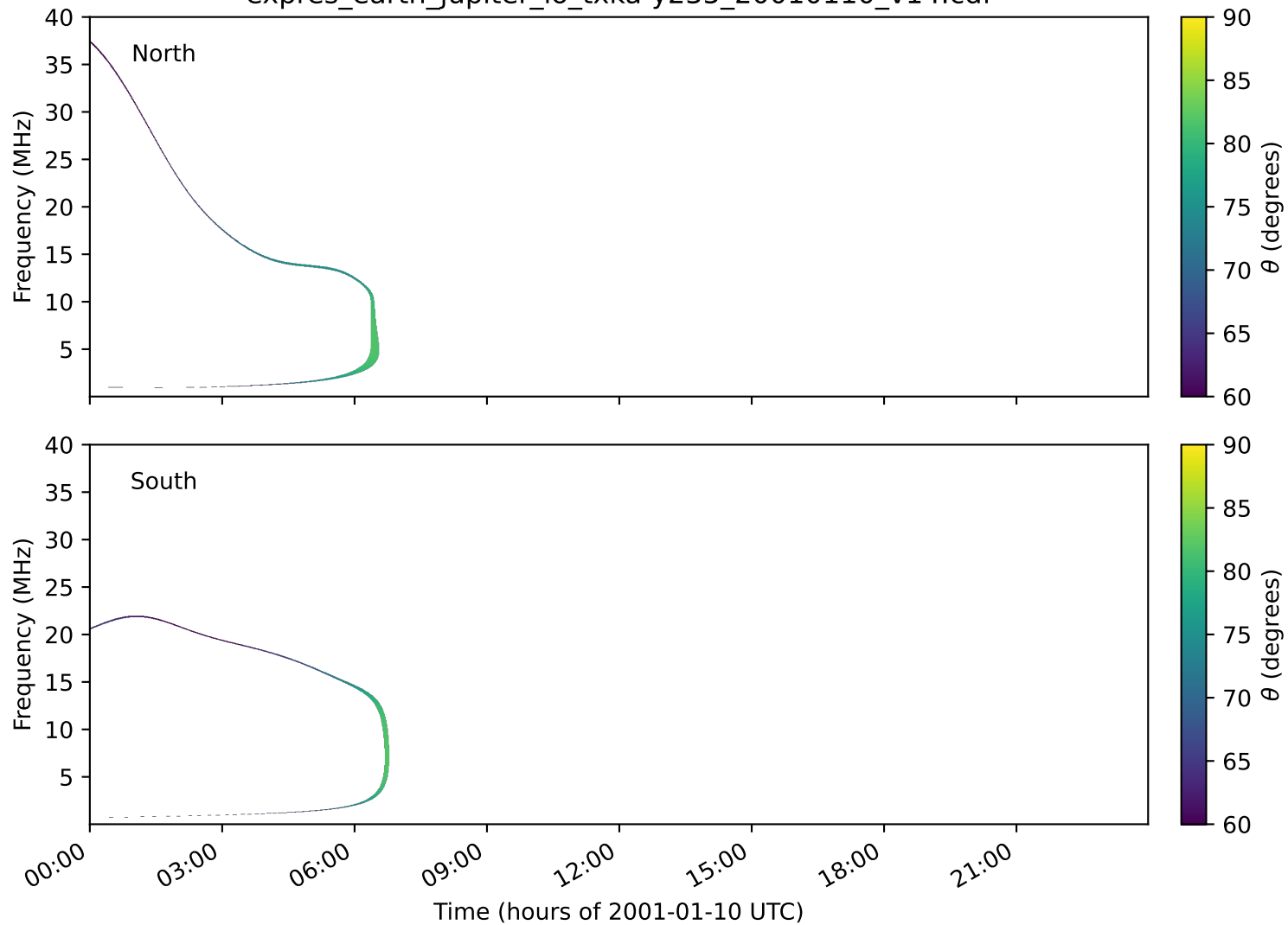
expres_earth_jupiter_io_txka-y235_20010110_v14.cdf
