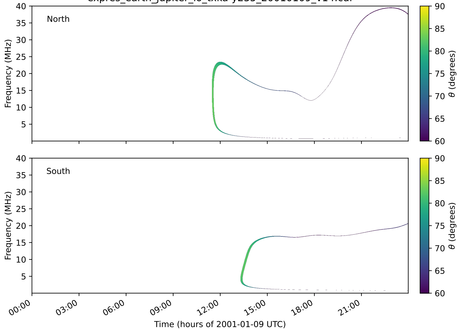
expres_earth_jupiter_io_txka-y235_20010109_v14.cdf
