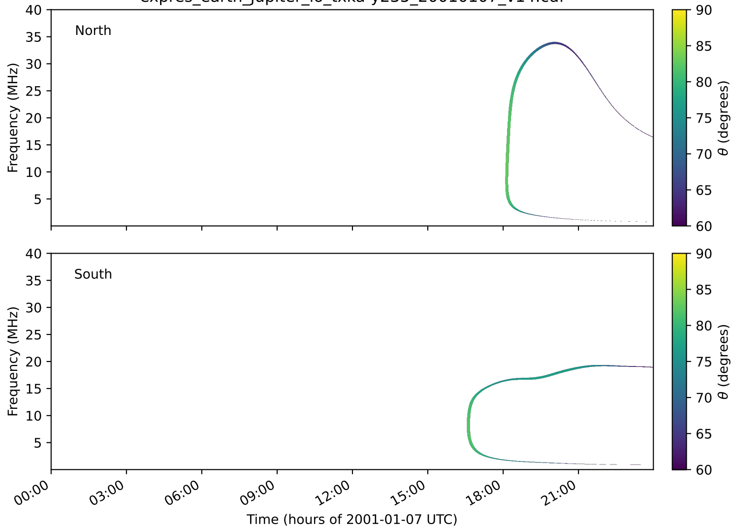
expres_earth_jupiter_io_txka-y235_20010107_v14.cdf
