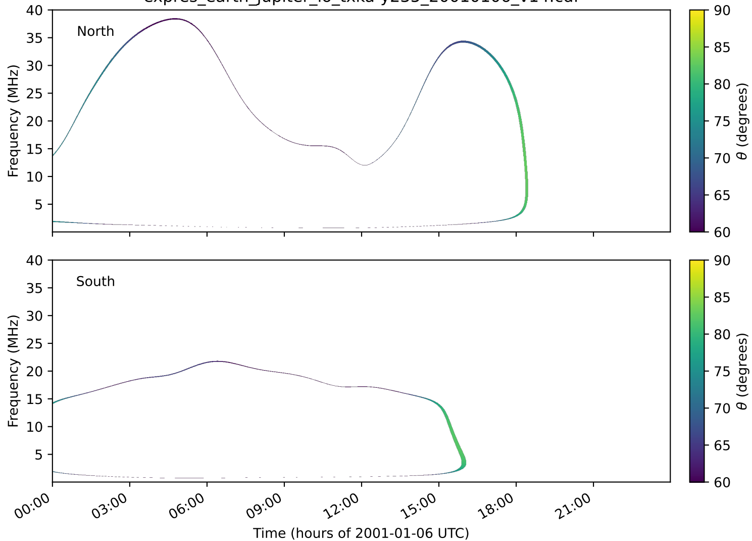
expres_earth_jupiter_io_txka-y235_20010106_v14.cdf
