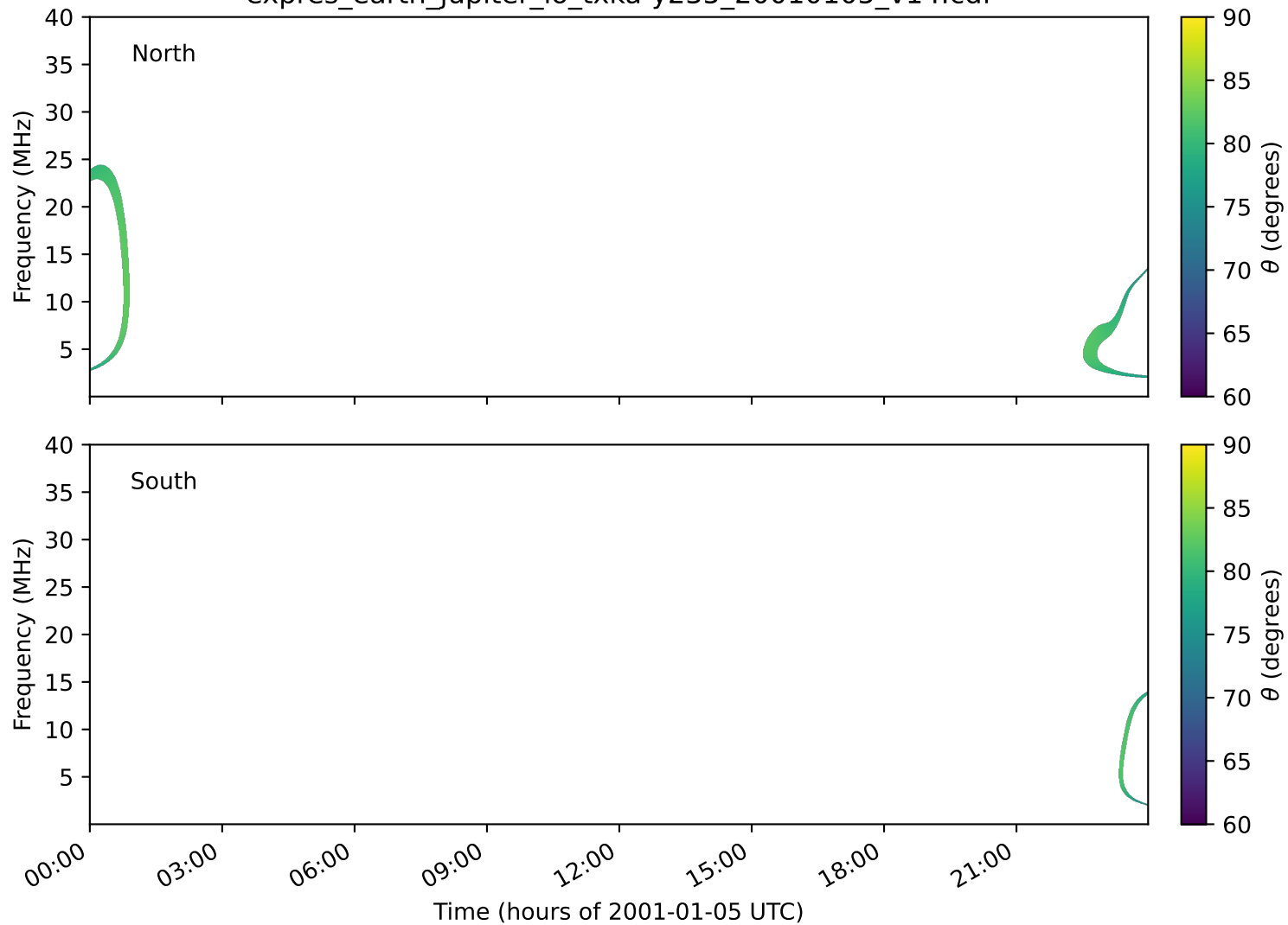
expres_earth_jupiter_io_txka-y235_20010105_v14.cdf
