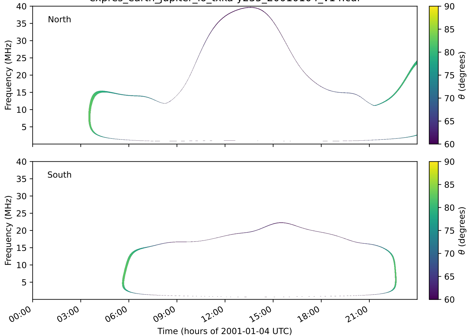
expres_earth_jupiter_io_txka-y235_20010104_v14.cdf
