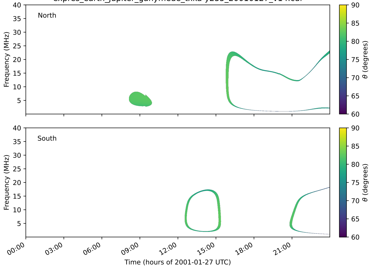
expres_earth_jupiter_ganymede_txka-y235_20010127_v14.cdf
