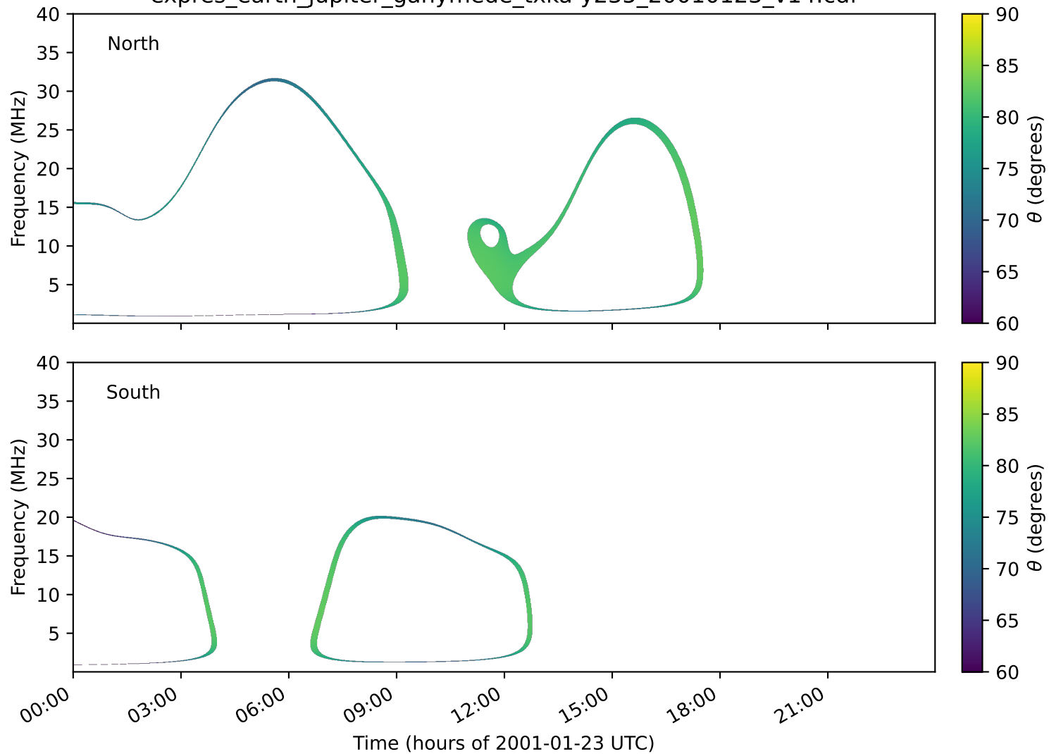
expres_earth_jupiter_ganymede_txka-y235_20010123_v14.cdf
