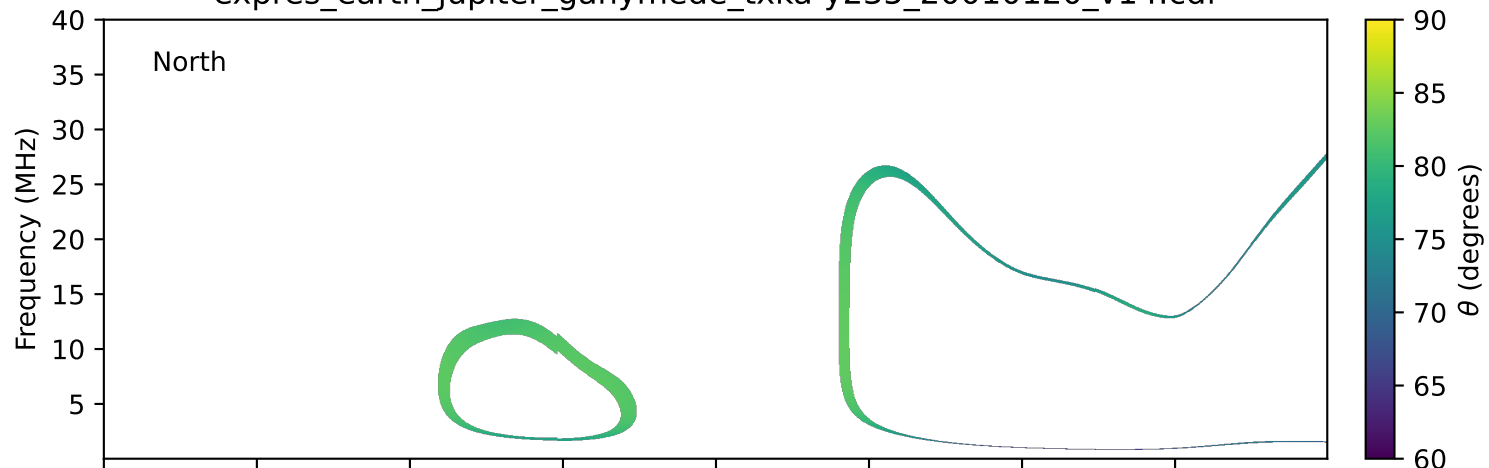
expres_earth_jupiter_ganymede_txka-y235_20010120_v14.cdf
