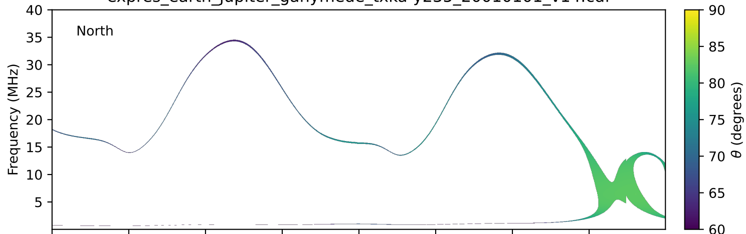
expres_earth_jupiter_ganymede_txka-y235_20010101_v14.cdf
