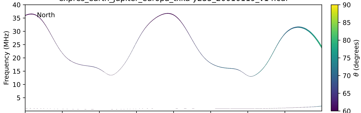
expres_earth_jupiter_europa_txka-y235_20010119_v14.cdf
