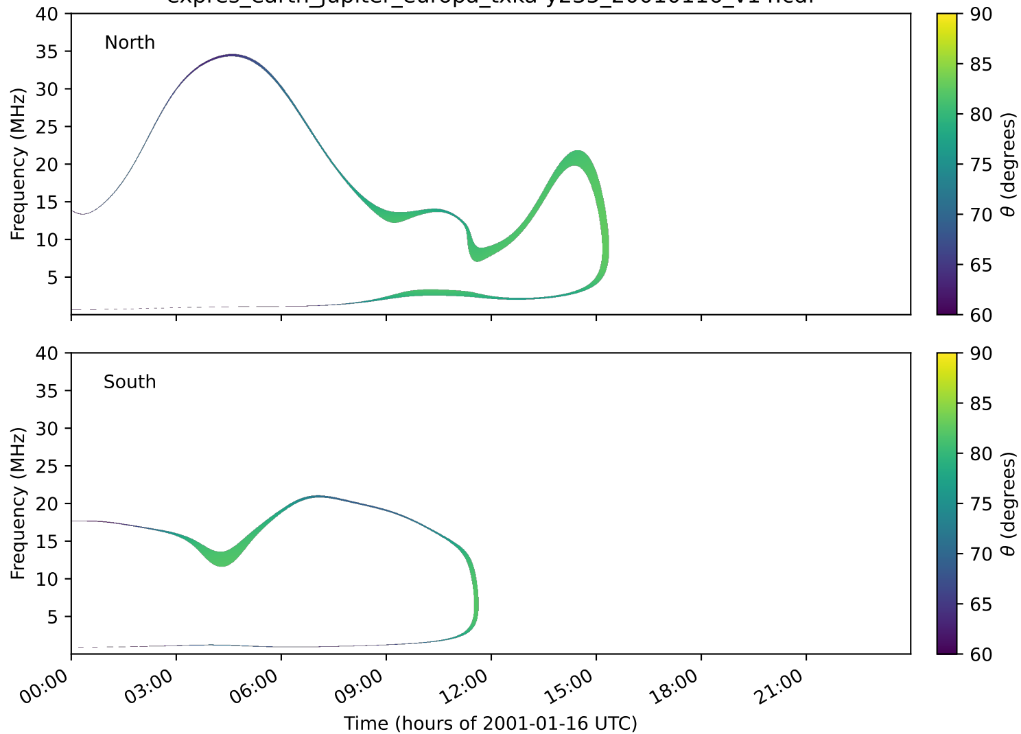
expres_earth_jupiter_europa_txka-y235_20010116_v14.cdf
