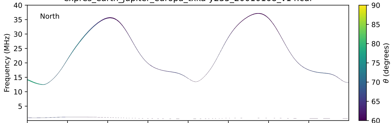
expres_earth_jupiter_europa_txka-y235_20010108_v14.cdf
