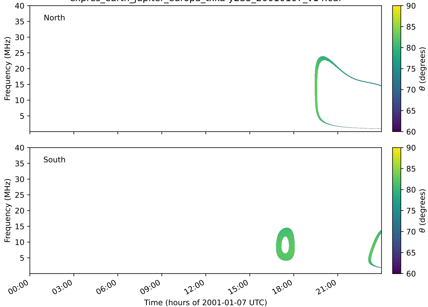
expres_earth_jupiter_europa_txka-y235_20010107_v14.cdf
