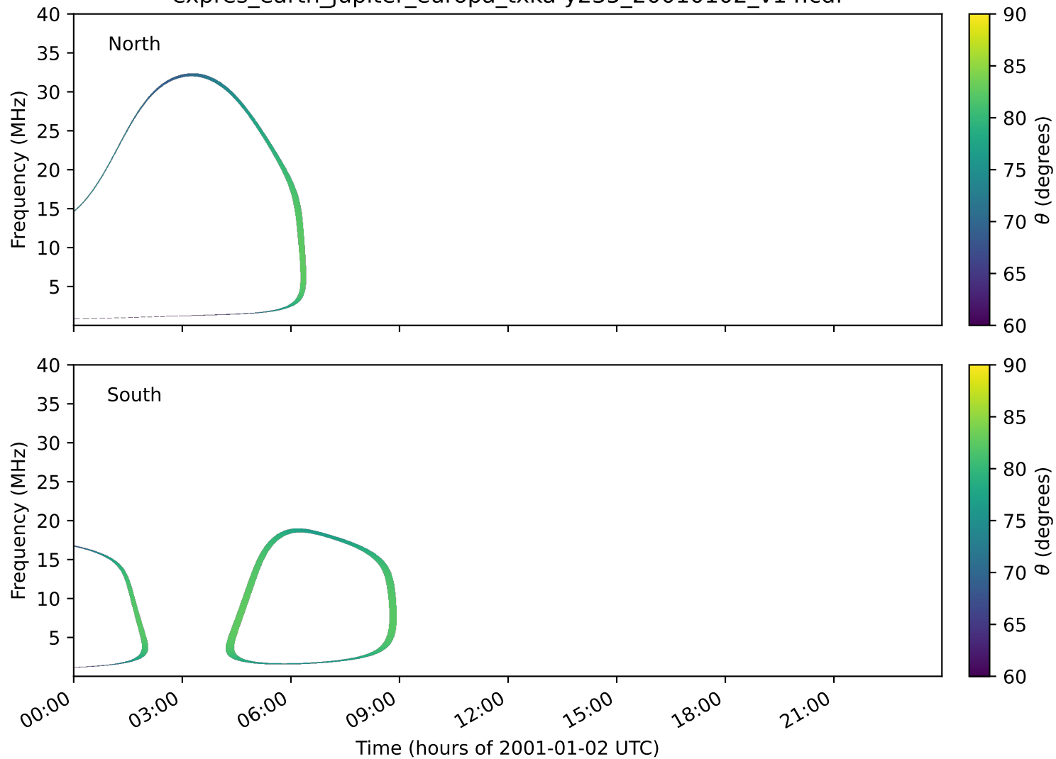
expres_earth_jupiter_europa_txka-y235_20010102_v14.cdf
