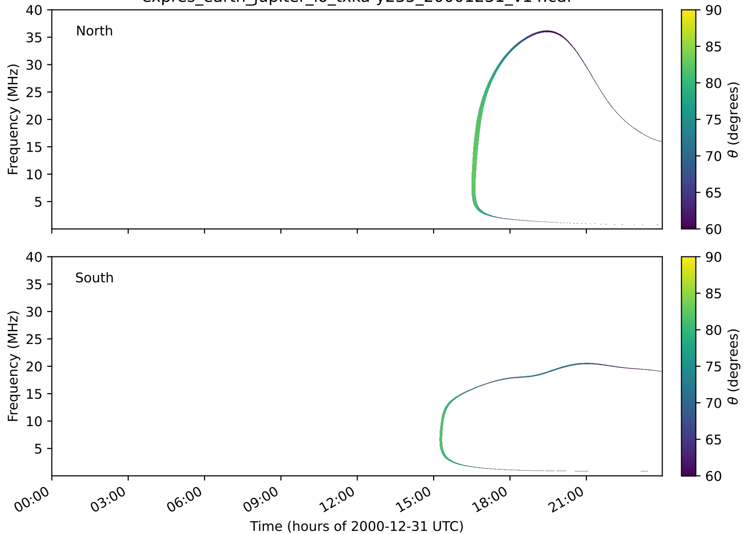
expres_earth_jupiter_io_txka-y235_20001231_v14.cdf
