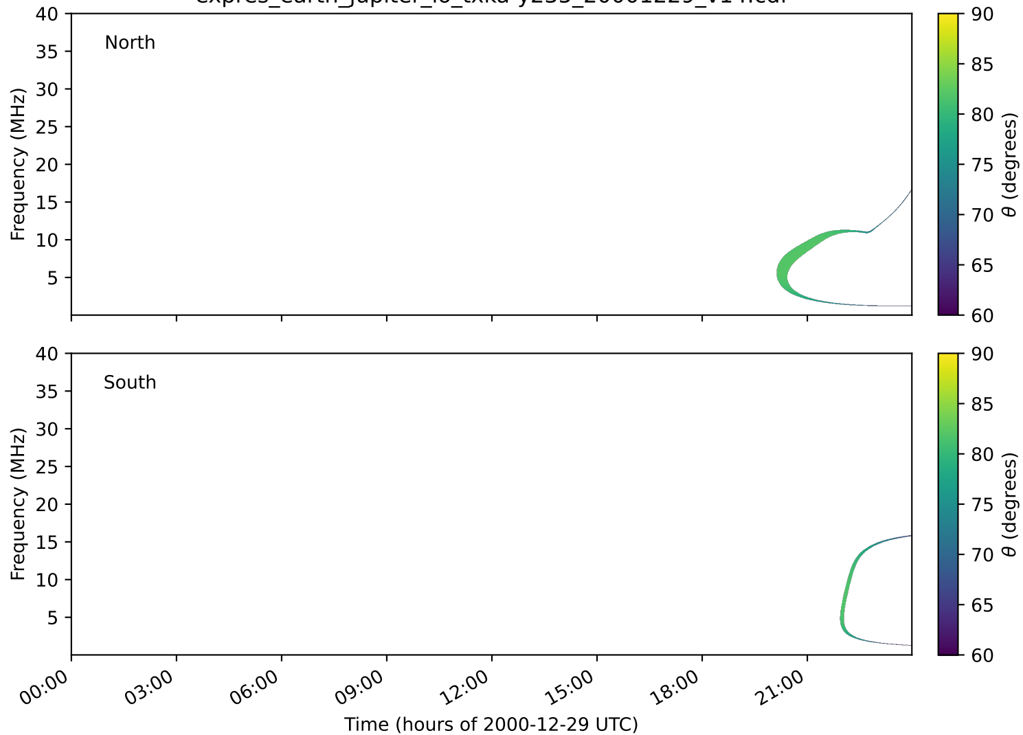
expres_earth_jupiter_io_txka-y235_20001229_v14.cdf
