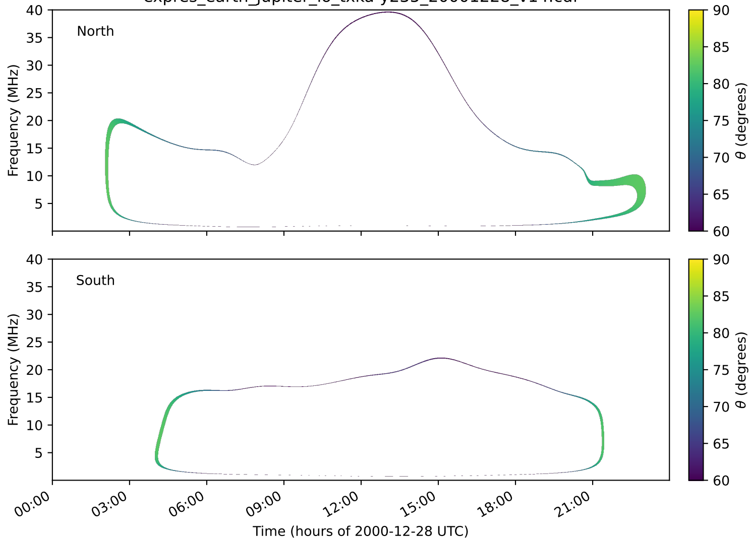
expres_earth_jupiter_io_txka-y235_20001228_v14.cdf
