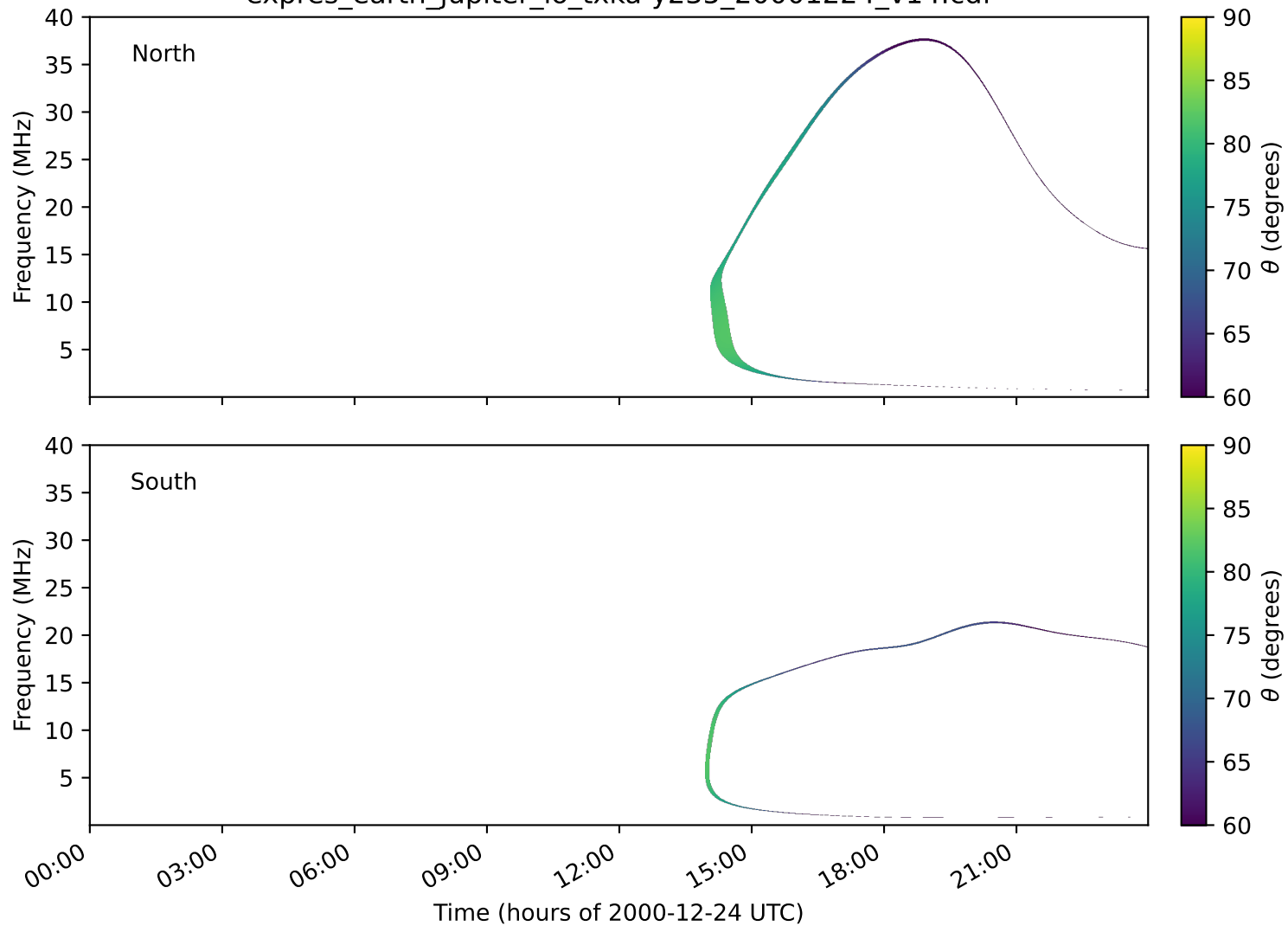
expres_earth_jupiter_io_txka-y235_20001224_v14.cdf
