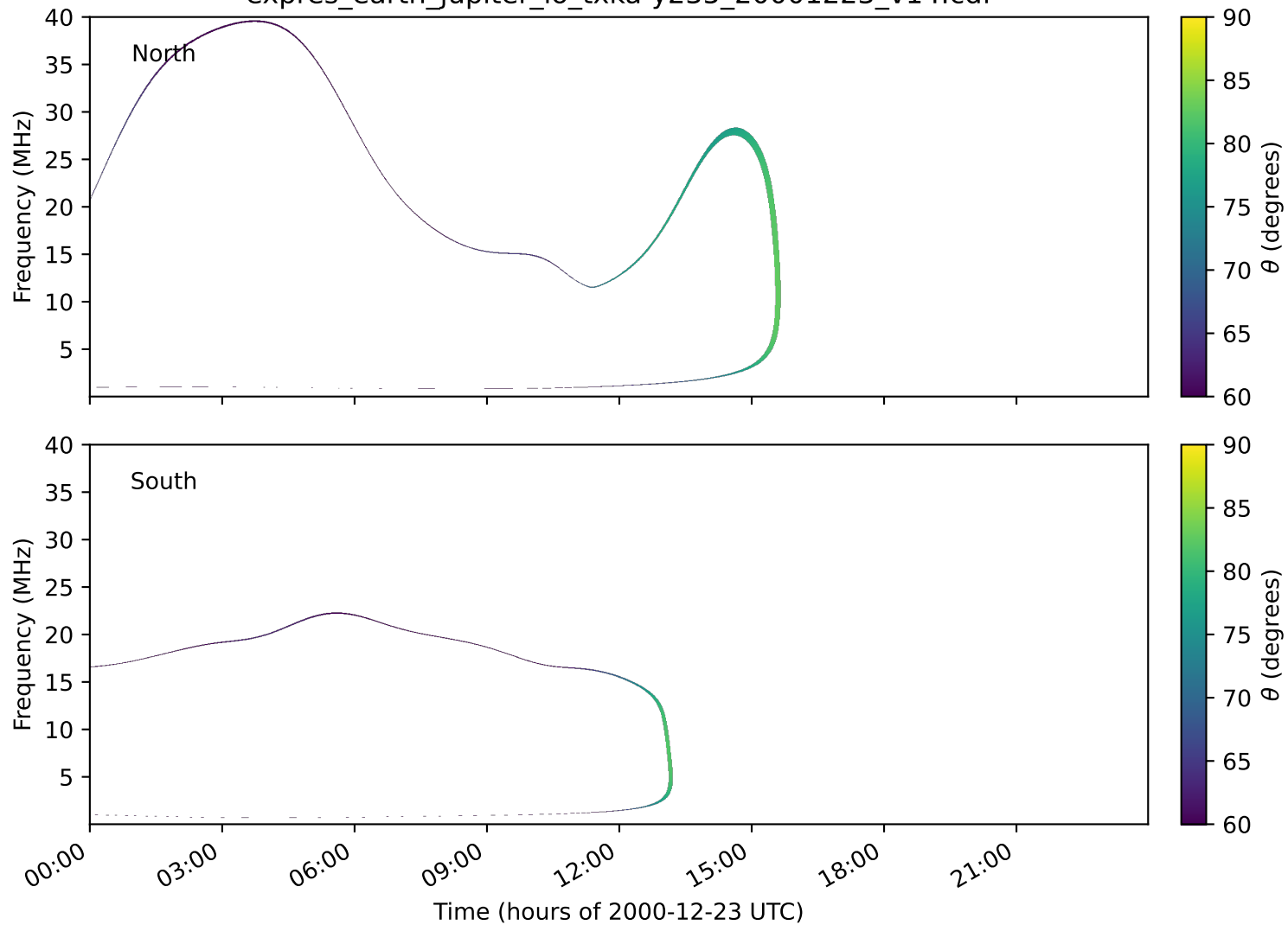
expres_earth_jupiter_io_txka-y235_20001223_v14.cdf
