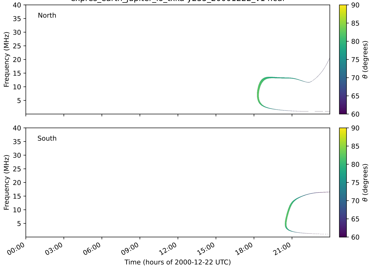
expres_earth_jupiter_io_txka-y235_20001222_v14.cdf
