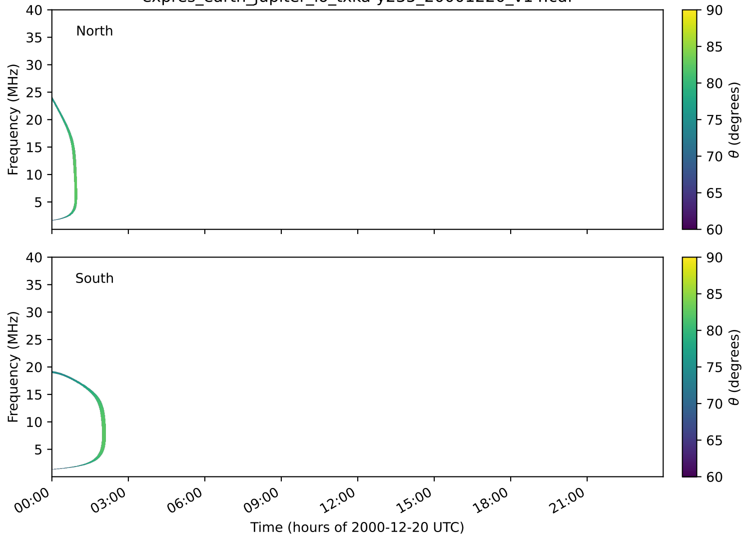
expres_earth_jupiter_io_txka-y235_20001220_v14.cdf
