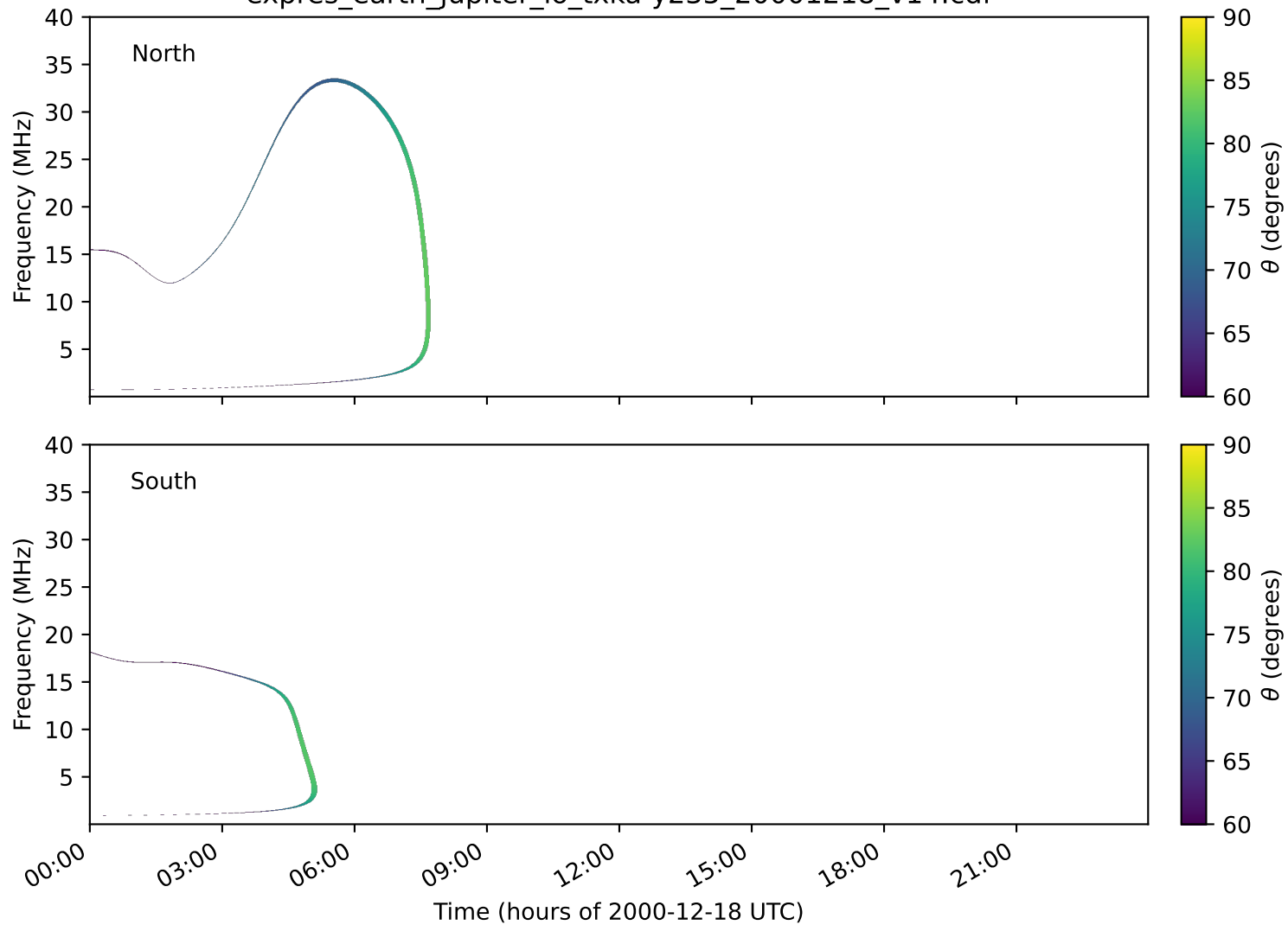
expres_earth_jupiter_io_txka-y235_20001218_v14.cdf
