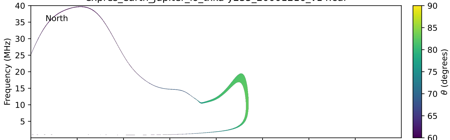
expres_earth_jupiter_io_txka-y235_20001216_v14.cdf
