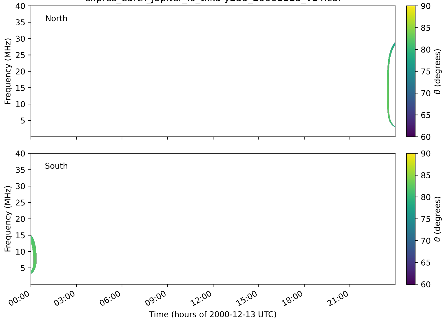
expres_earth_jupiter_io_txka-y235_20001213_v14.cdf
