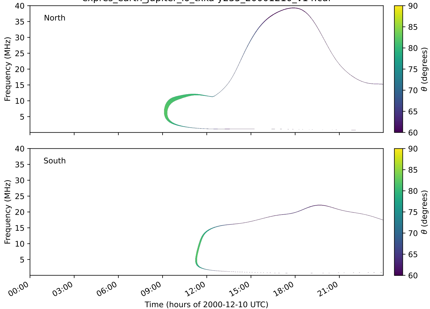
expres_earth_jupiter_io_txka-y235_20001210_v14.cdf
