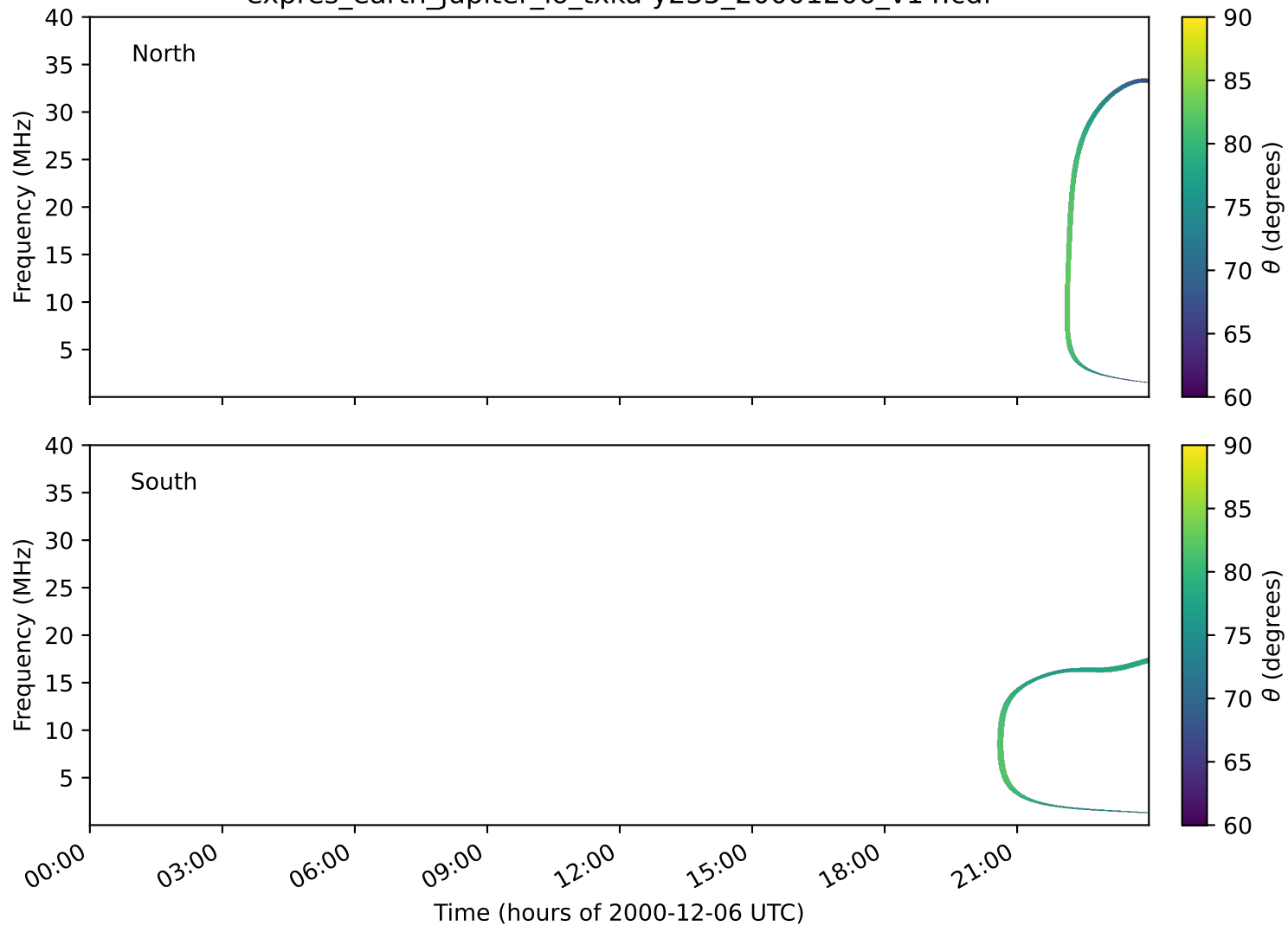
expres_earth_jupiter_io_txka-y235_20001206_v14.cdf
