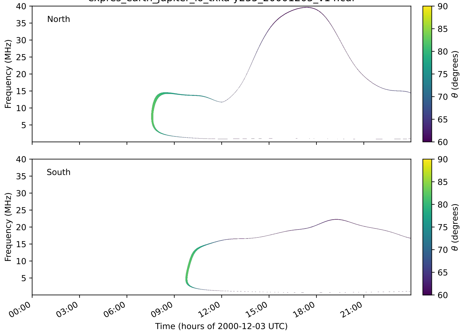
expres_earth_jupiter_io_txka-y235_20001203_v14.cdf
