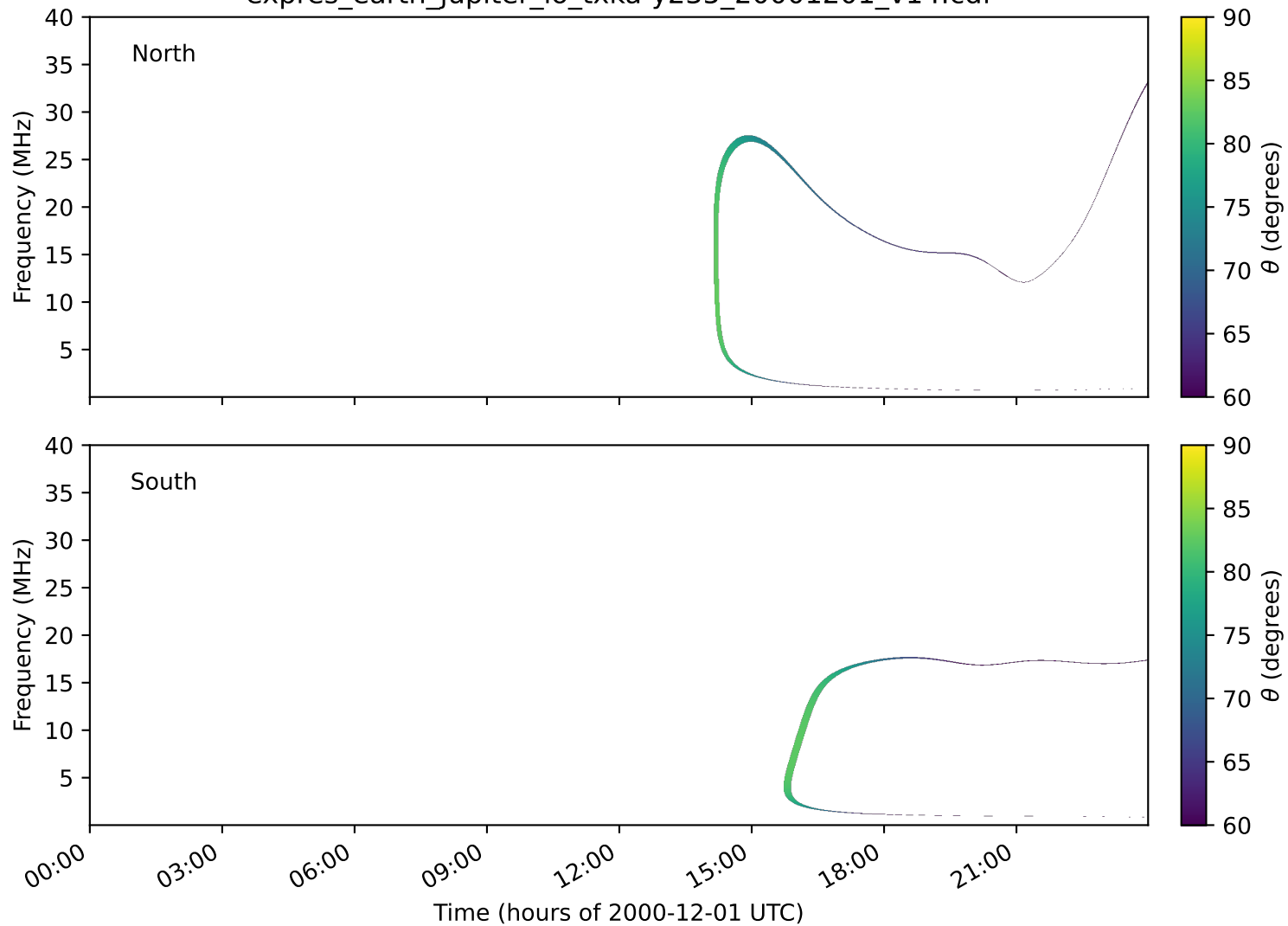
expres_earth_jupiter_io_txka-y235_20001201_v14.cdf
