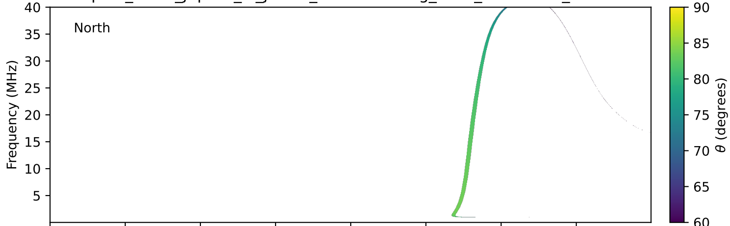
expres_earth_jupiter_io_jrm33_lossc-wid1deg_3kev_20001231_v11.cdf
