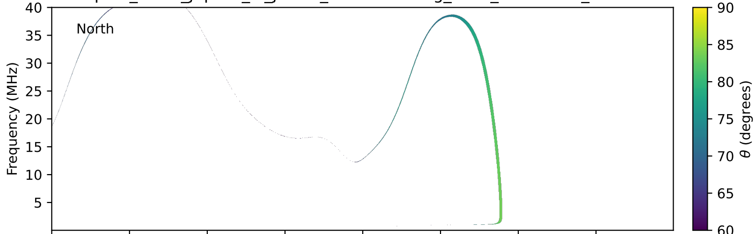
expres_earth_jupiter_io_jrm33_lossc-wid1deg_3kev_20001230_v11.cdf
