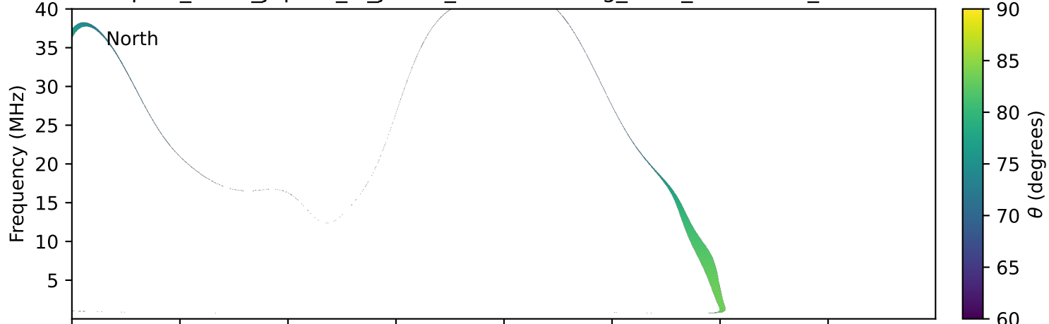
expres_earth_jupiter_io_jrm33_lossc-wid1deg_3kev_20001214_v11.cdf
