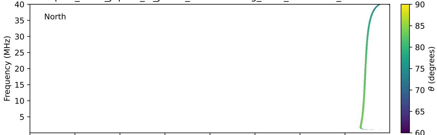
expres_earth_jupiter_io_jrm33_lossc-wid1deg_3kev_20001206_v11.cdf
