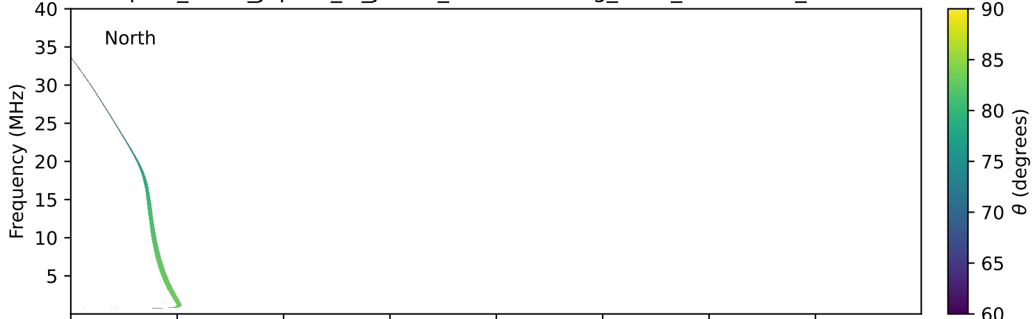
expres_earth_jupiter_io_jrm09_lossc-wid1deg_3kev_20001227_v11.cdf
