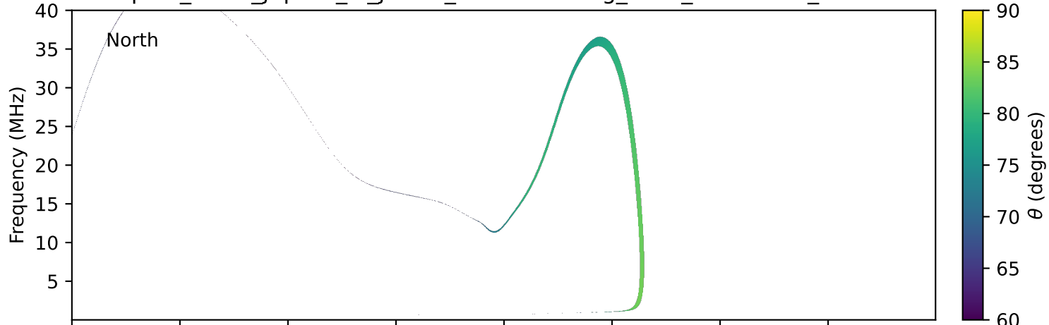
expres_earth_jupiter_io_jrm09_lossc-wid1deg_3kev_20001223_v11.cdf
