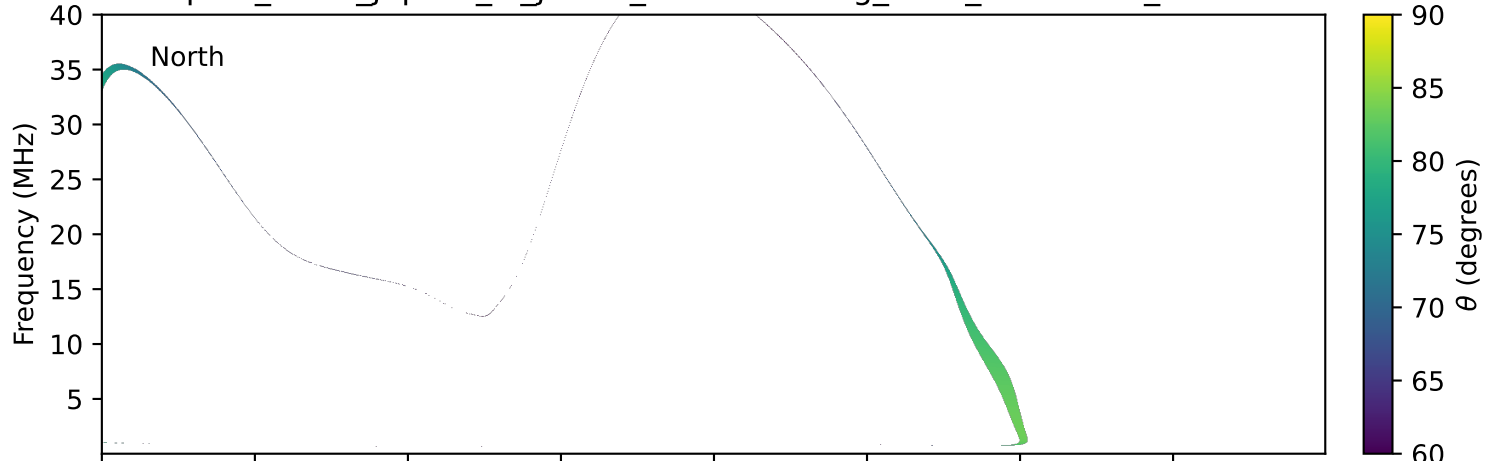
expres_earth_jupiter_io_jrm09_lossc-wid1deg_3kev_20001214_v11.cdf
