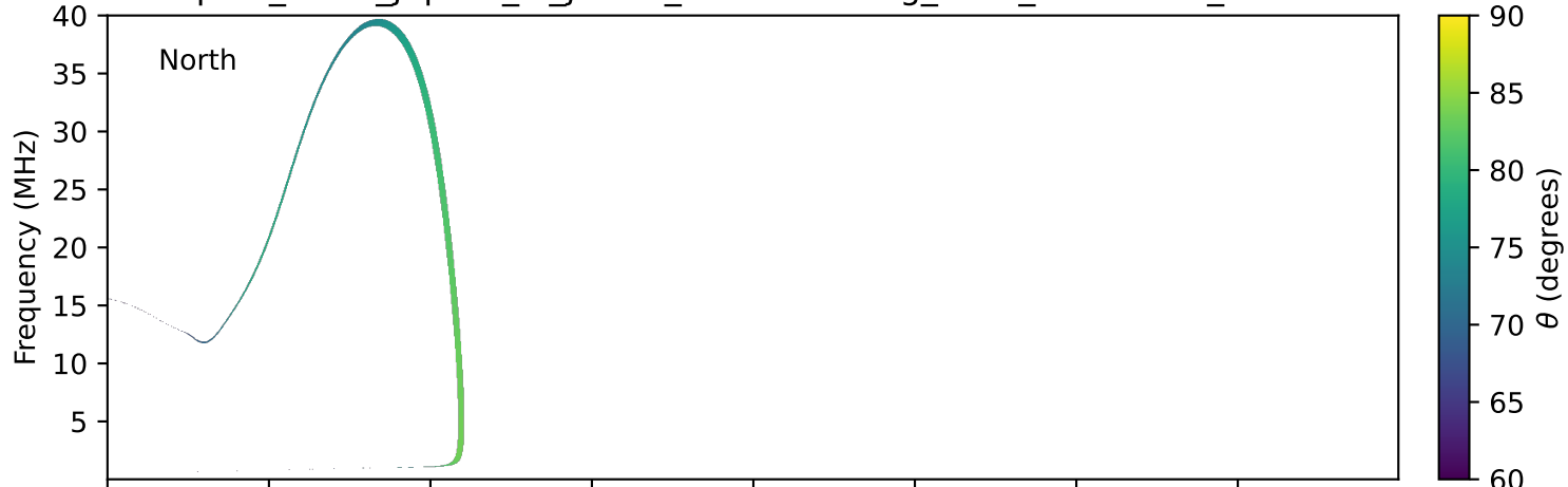
expres_earth_jupiter_io_jrm09_lossc-wid1deg_3kev_20001211_v11.cdf
