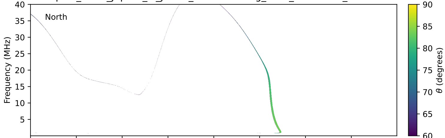
expres_earth_jupiter_io_jrm09_lossc-wid1deg_3kev_20001207_v11.cdf
