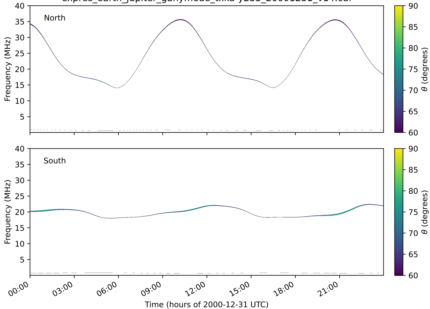
expres_earth_jupiter_ganymede_txka-y235_20001231_v14.cdf
