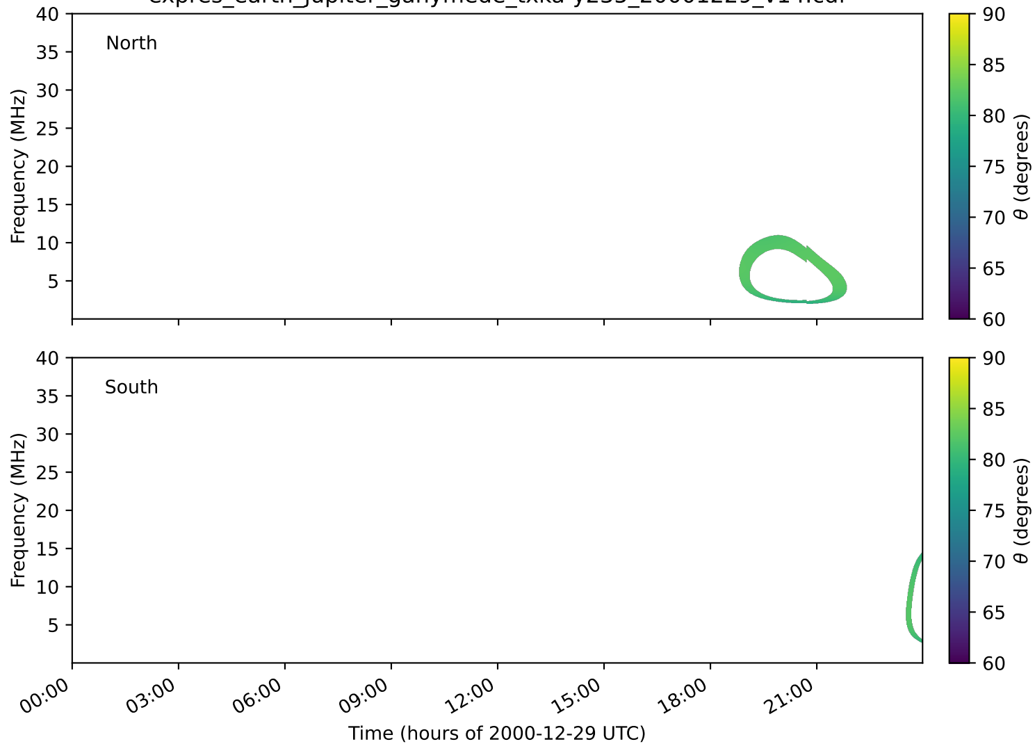
expres_earth_jupiter_ganymede_txka-y235_20001229_v14.cdf
