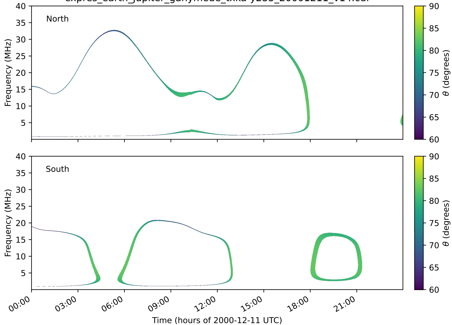
expres_earth_jupiter_ganymede_txka-y235_20001211_v14.cdf
