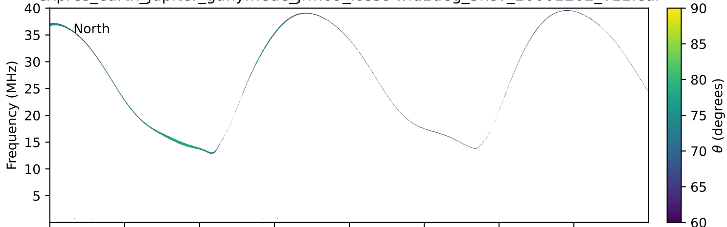
expres_earth_jupiter_ganymede_jrm09_lossc-wid1deg_3kev_20001202_v11.cdf
