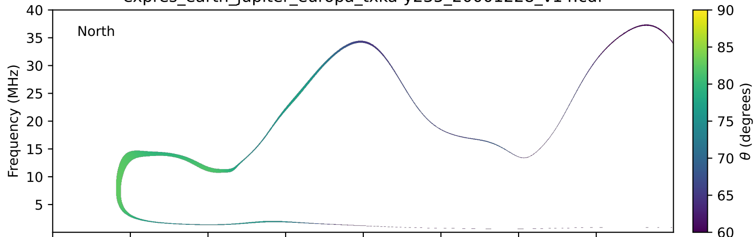
expres_earth_jupiter_europa_txka-y235_20001228_v14.cdf
