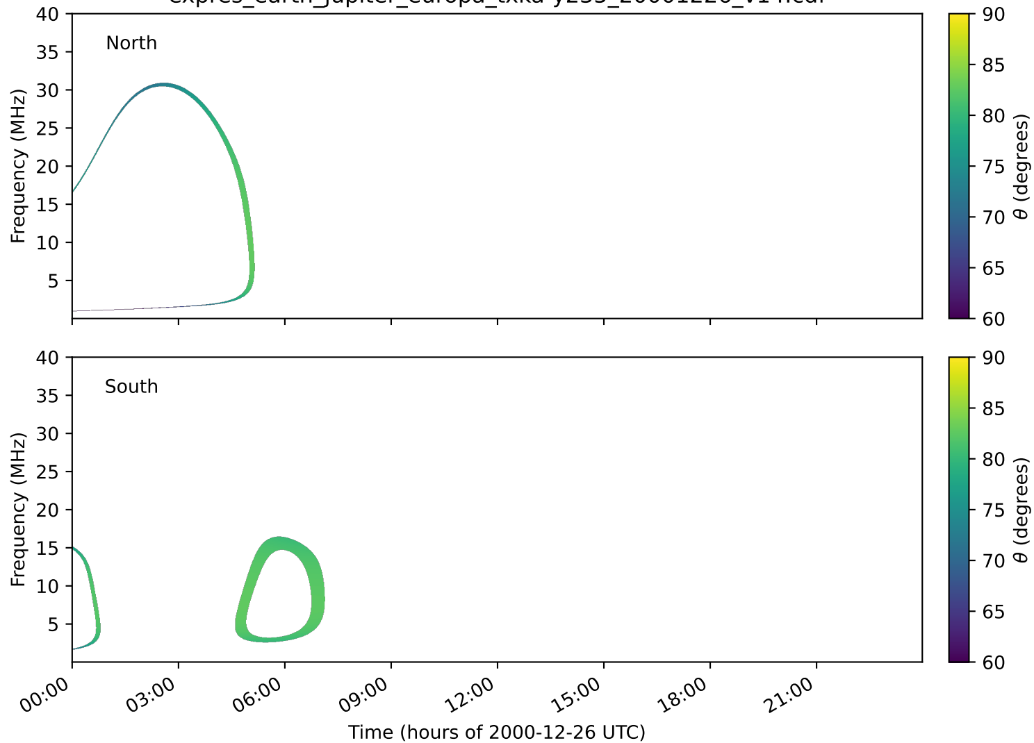
expres_earth_jupiter_europa_txka-y235_20001226_v14.cdf
