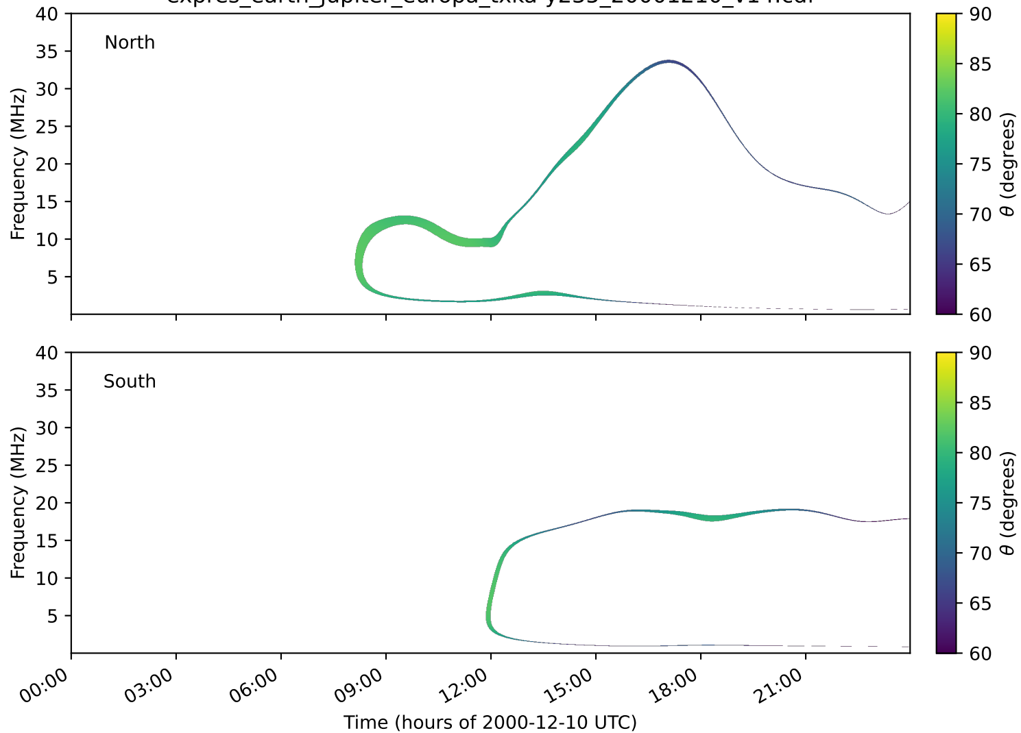
expres_earth_jupiter_europa_txka-y235_20001210_v14.cdf
