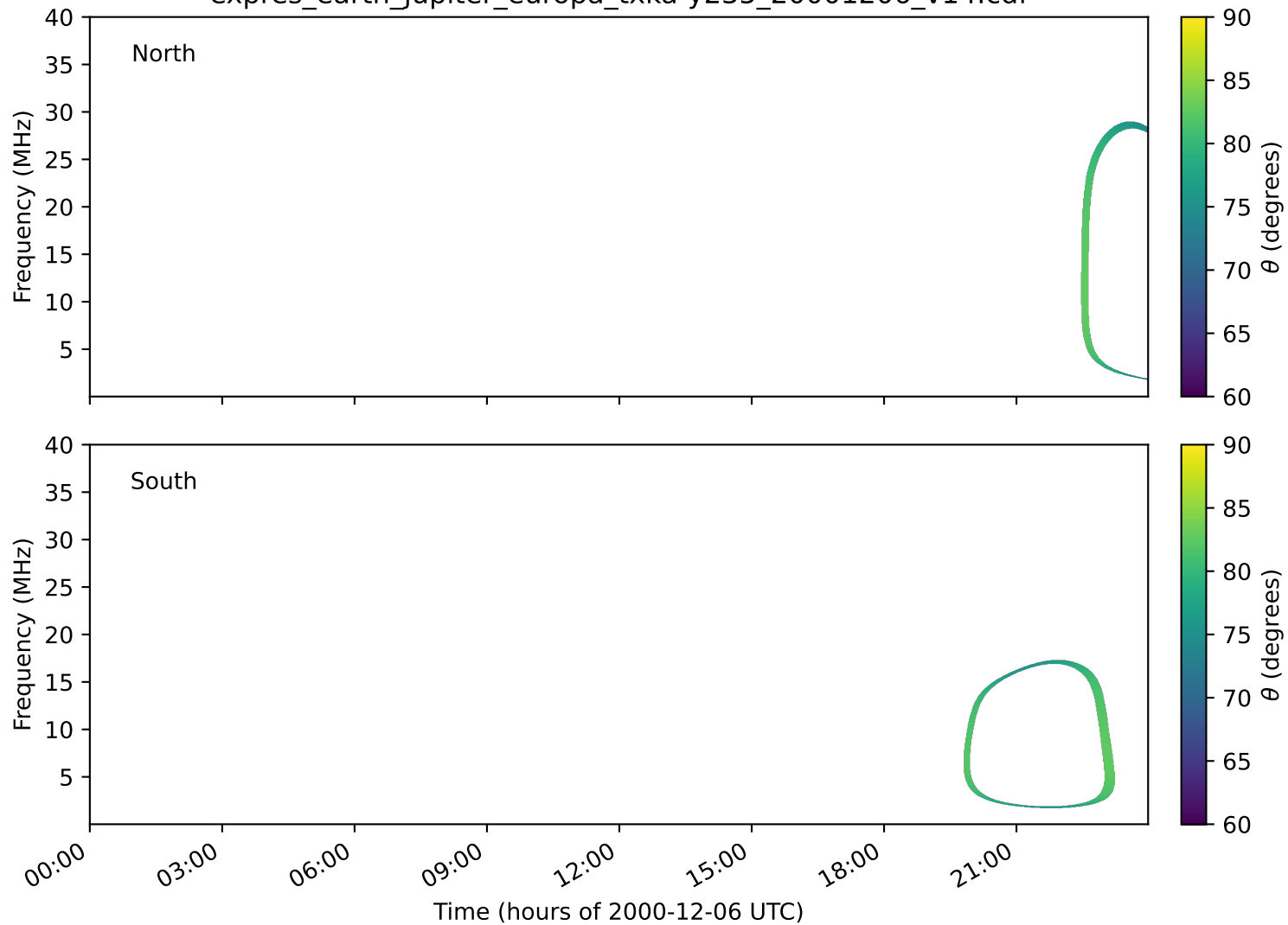
expres_earth_jupiter_europa_txka-y235_20001206_v14.cdf
